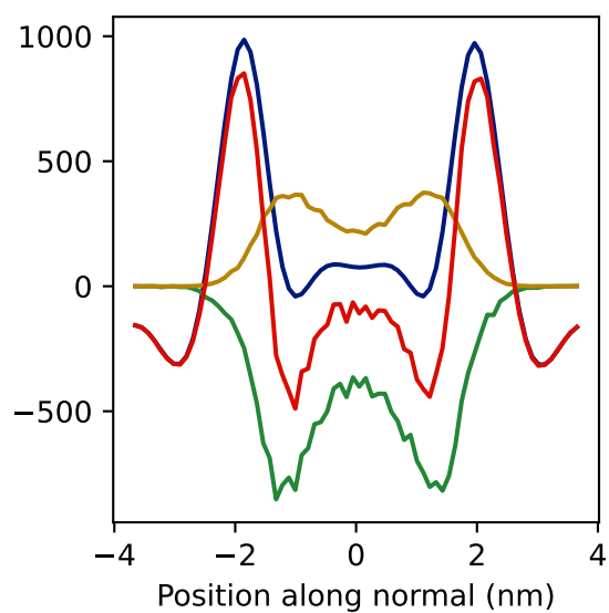
DPPG
