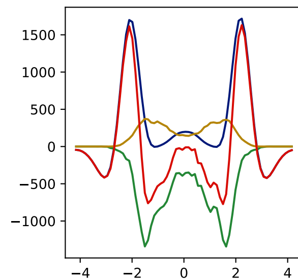
POPE
