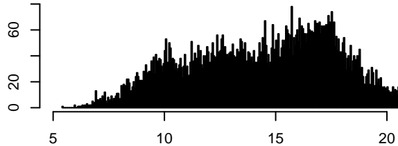
Closed Holo Simulations
