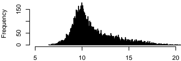
Closed Apo Simulations
