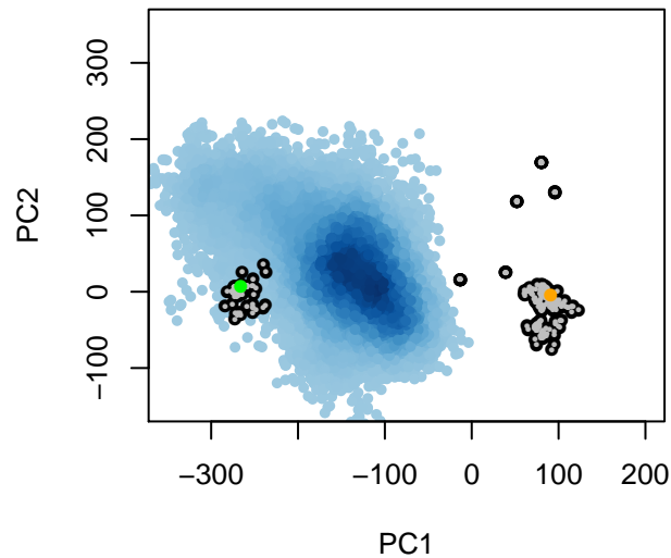
Open Holo
