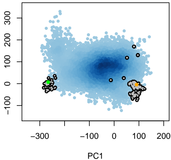
Closed Holo
