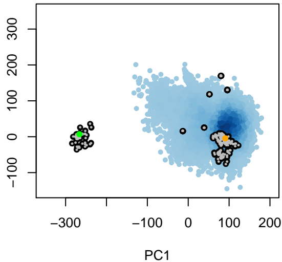
Closed Apo
