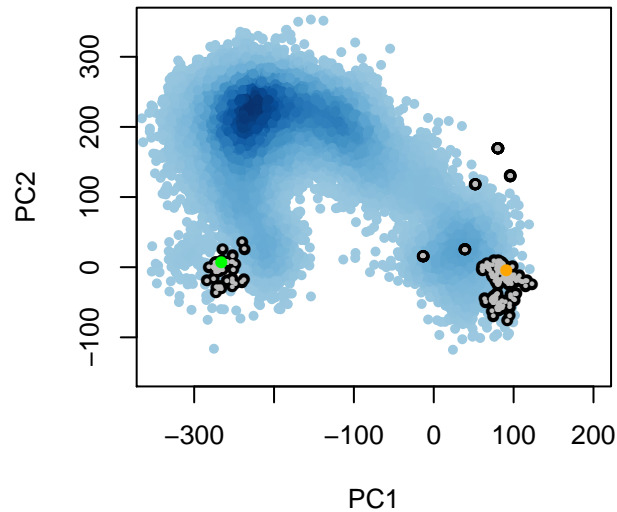
Open Apo
