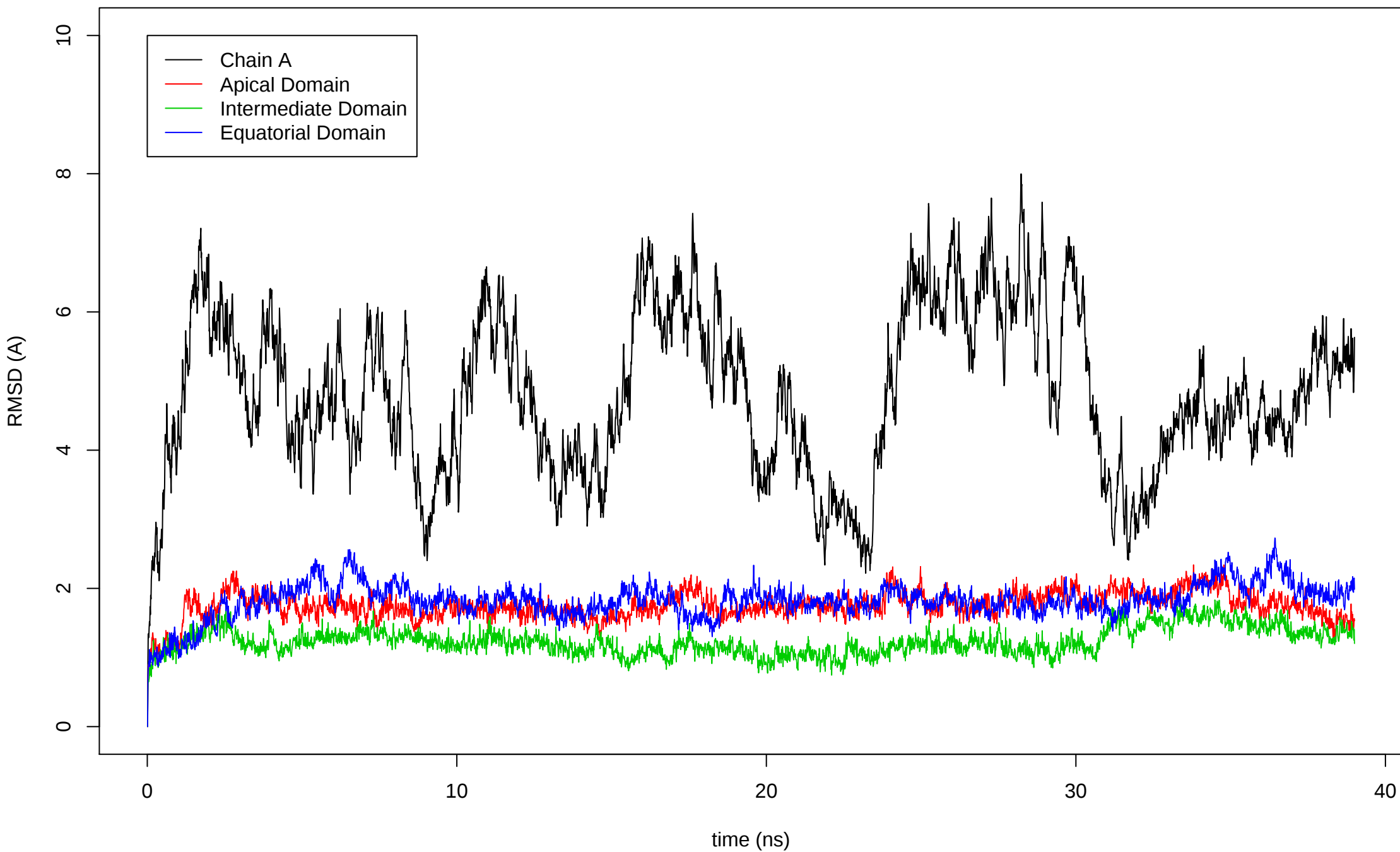
RMSD of Chain A during simulation
