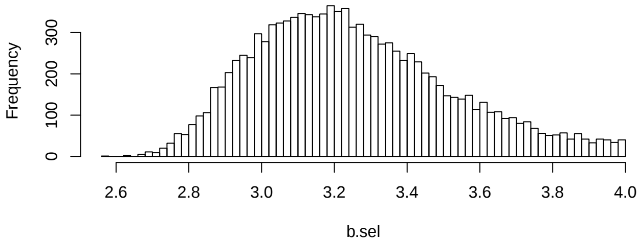
Histogram of b.sel
