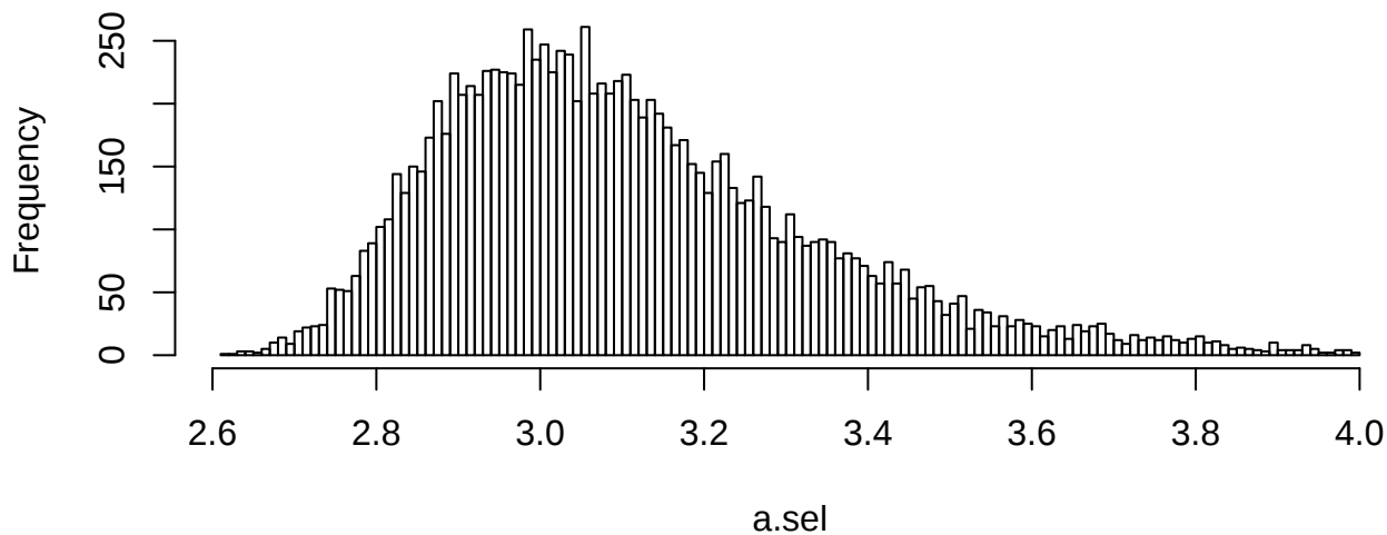
Histogram of a.sel
