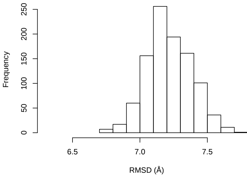
GroEL (ATP-free) cis ring
