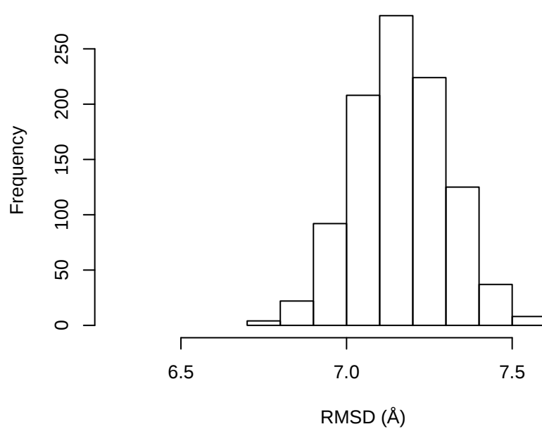
GroEL (ATP-free) trans ring
