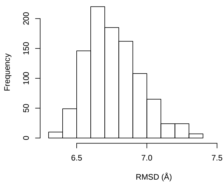
GroEL (Rhodanese ATP) cis ring
