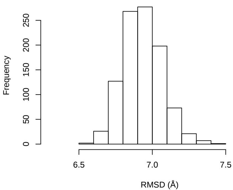
GroEL (ATP) cis ring
