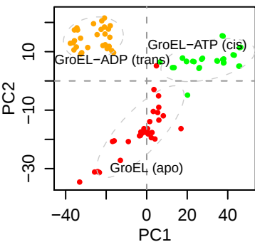
(C) GroEL ATP 7 (cis)
