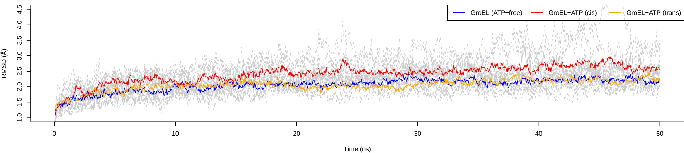
(A) Monomers
