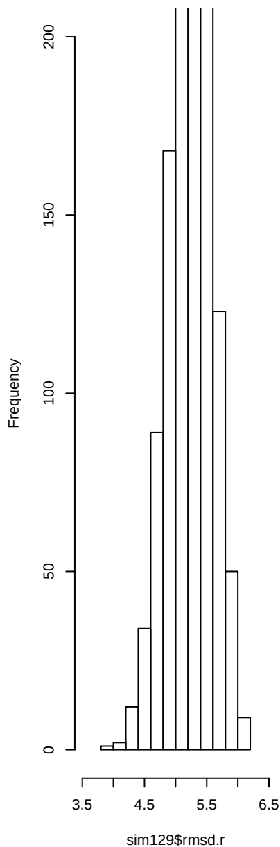
Histogram of sim129$rmsd.r
