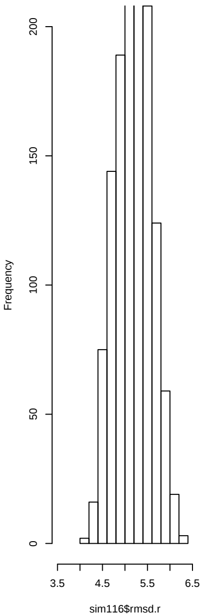
Histogram of sim116$rmsd.r
