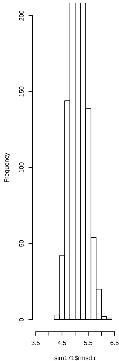
Histogram of sim171$rmsd.r
