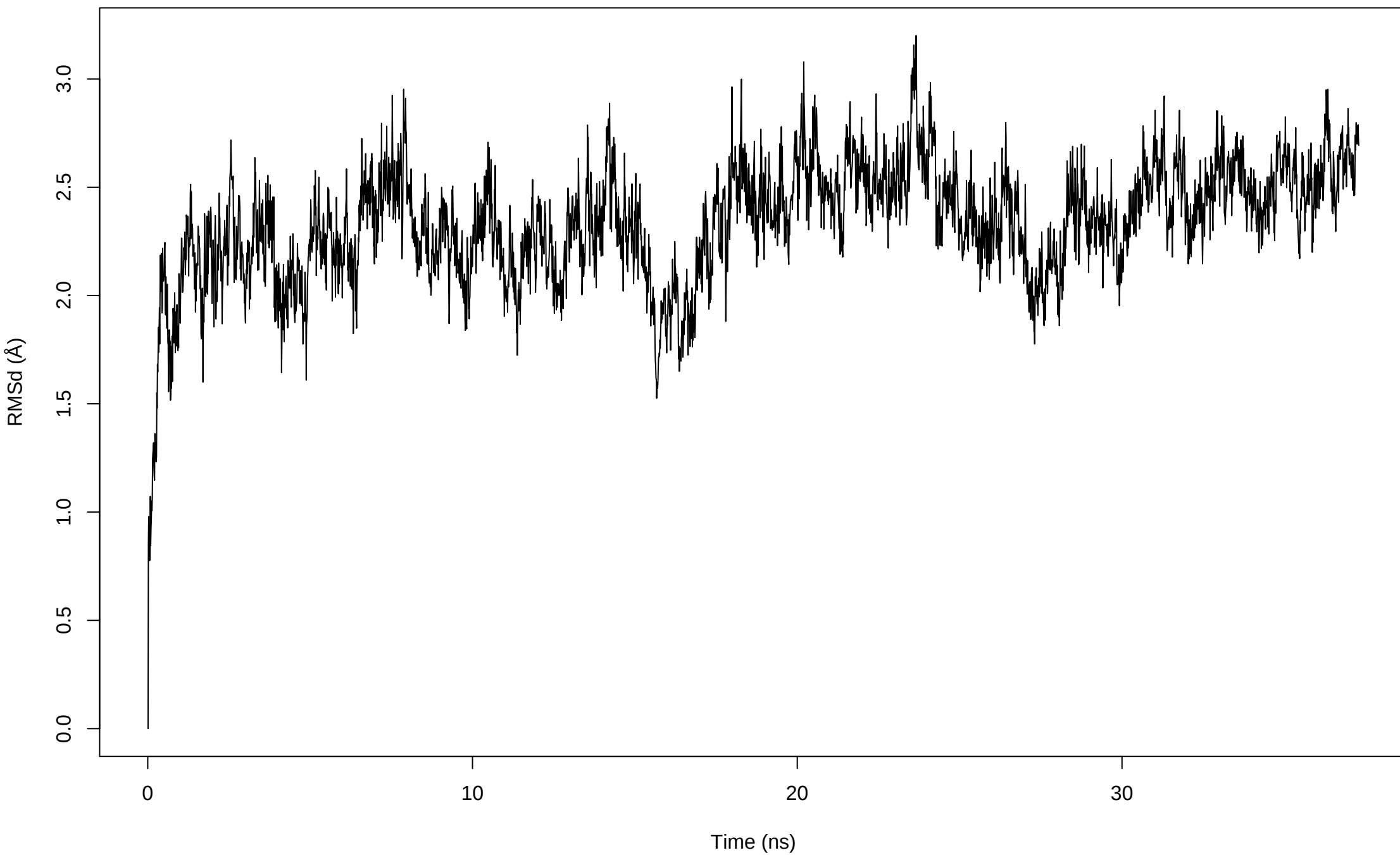
1XCK Chain A MgATP
