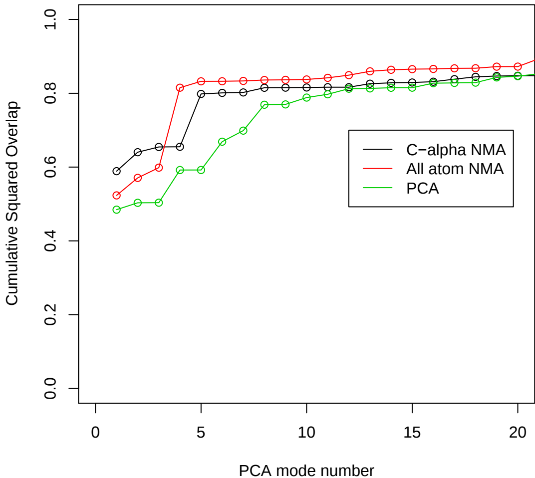
Cumulative Overlap values for NMA and PCA
