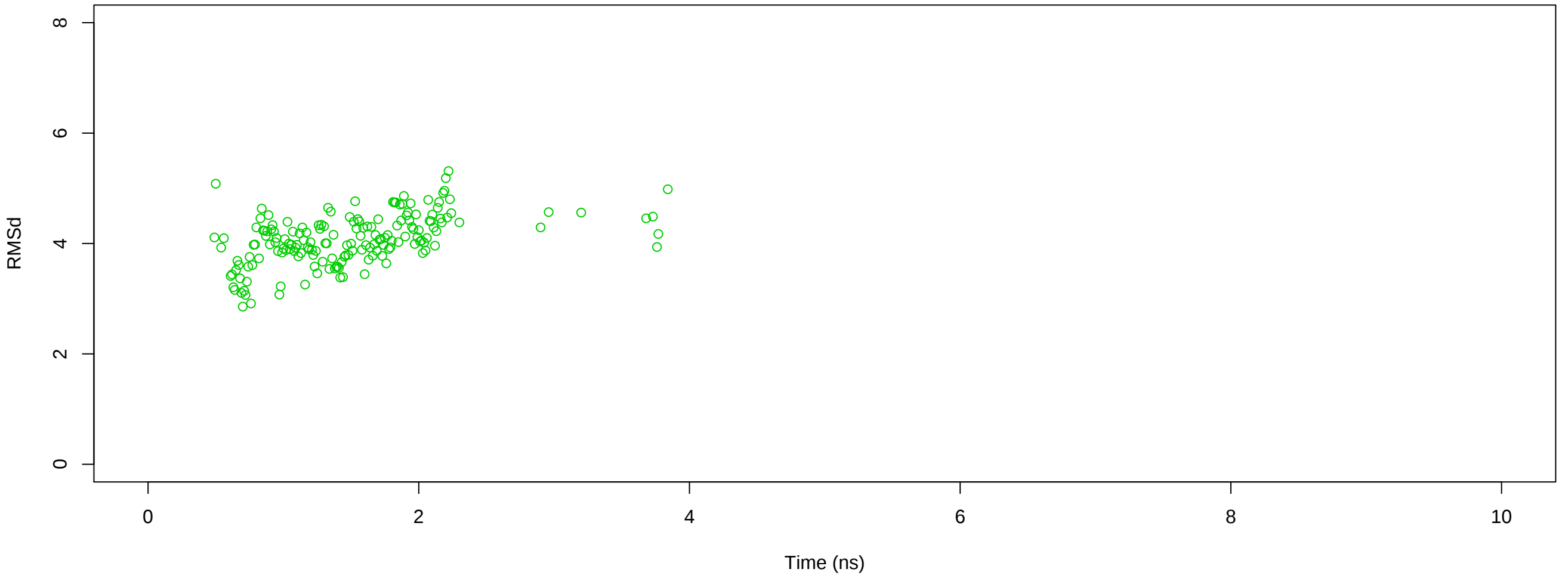
RMSd and clusters
