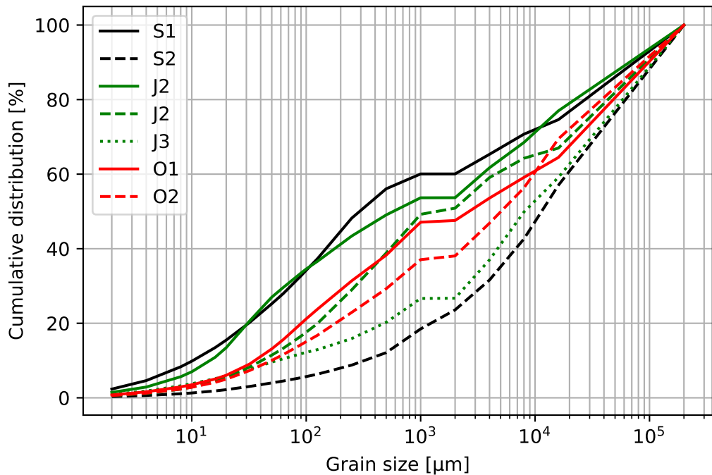
Grain size distribution
