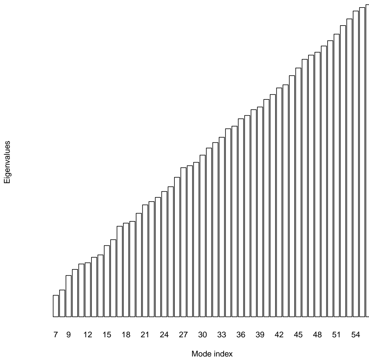
Eigenvalues plot for 1E15.pdb
