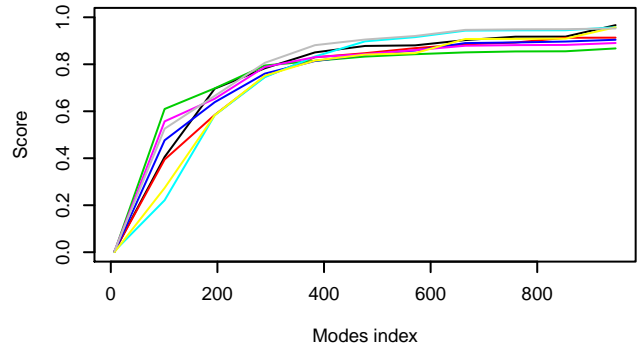
Cumulative overlap of CA modes of 3CWN (indiv_translation)
