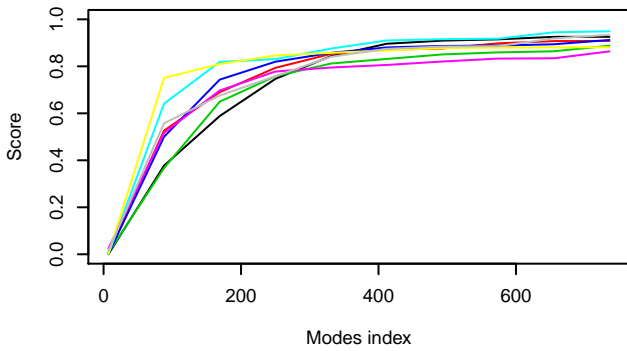
Cumulative overlap of CA modes of 3CH0 (indiv_translation)
