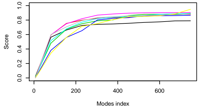
Cumulative overlap of CA modes of 1N55 (indiv_translation)
