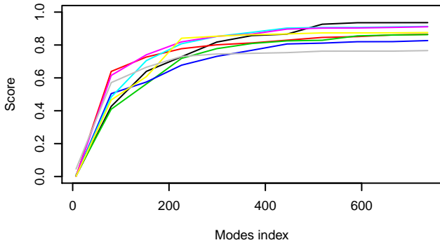
Cumulative overlap of CA modes of 1KKO (indiv_translation)
