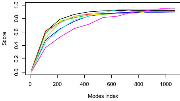
Cumulative overlap of CA modes of 1E15 (indiv_translation)
