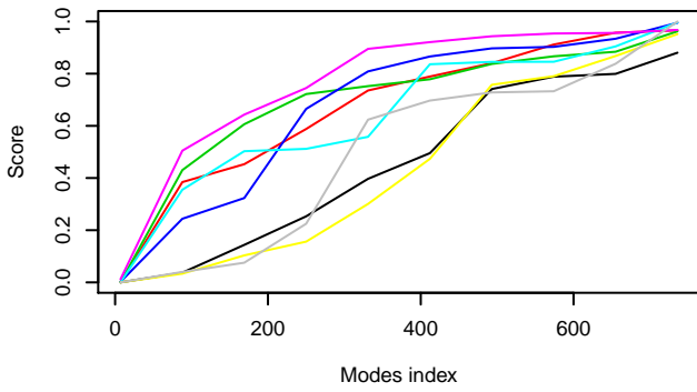
Cumulative overlap of CA modes of 3CH0 (indiv_tilt)
