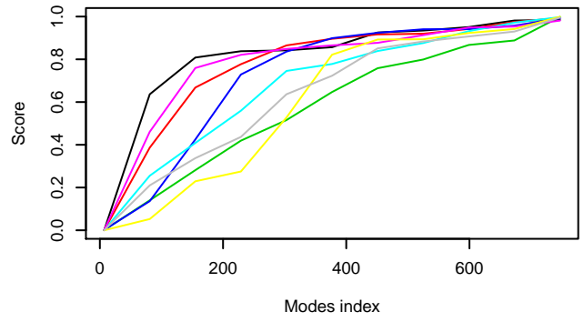
Cumulative overlap of CA modes of 1N55 (indiv_tilt)
