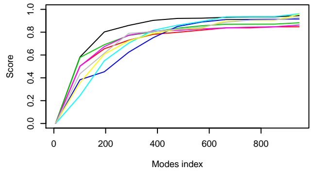
Cumulative overlap of CA modes of 3CWN (indiv_slide)
