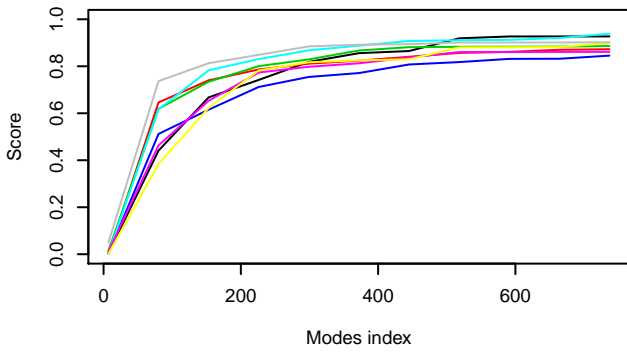
Cumulative overlap of CA modes of 1KKO (indiv_slide)
