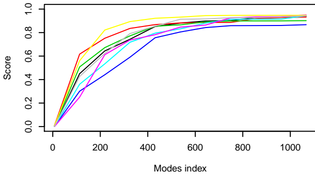
Cumulative overlap of CA modes of 1E15 (indiv_slide)
