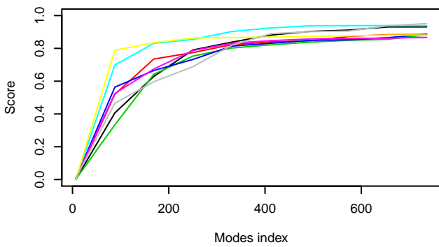
Cumulative overlap of CA modes of 3CH0 (indiv_slide)
