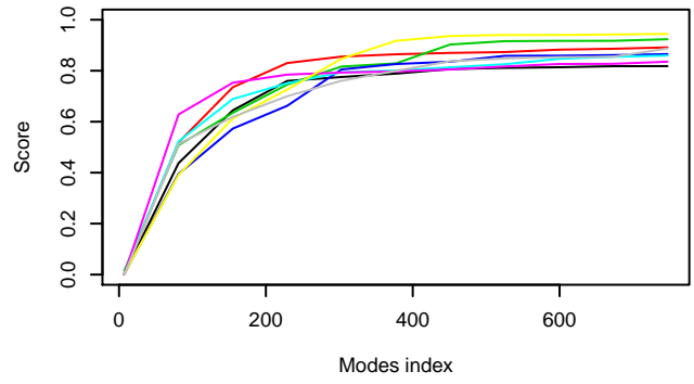
Cumulative overlap of CA modes of 1N55 (indiv_slide)
