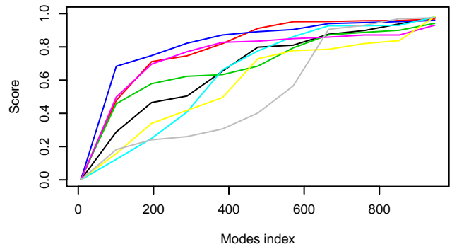
Cumulative overlap of CA modes of 3CWN (indiv_bend_upper)
