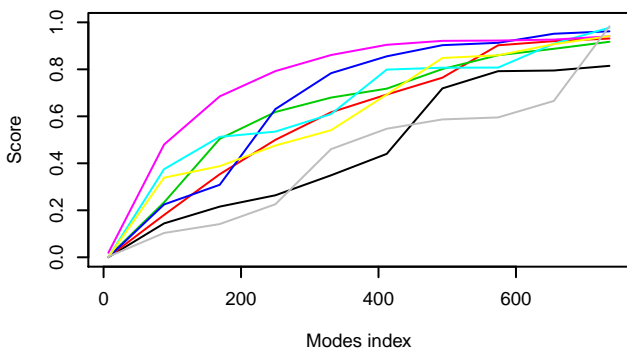
Cumulative overlap of CA modes of 3CH0 (indiv_bend_upper)
