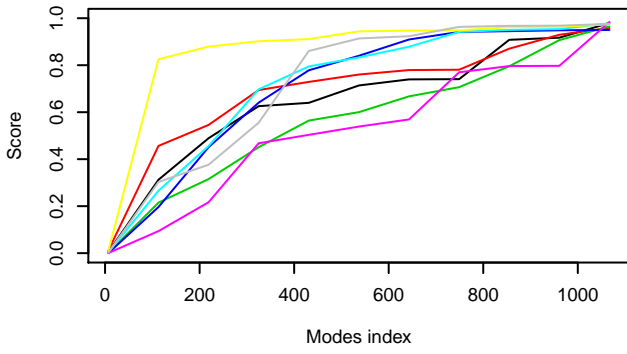
Cumulative overlap of CA modes of 1E15 (indiv_bend_upper)
