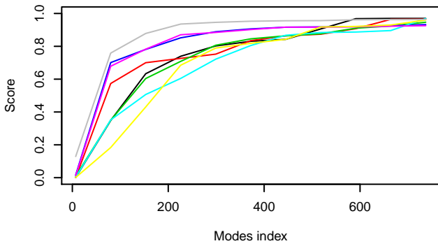
Cumulative overlap of CA modes of 1KKO (indiv_bend_upper)
