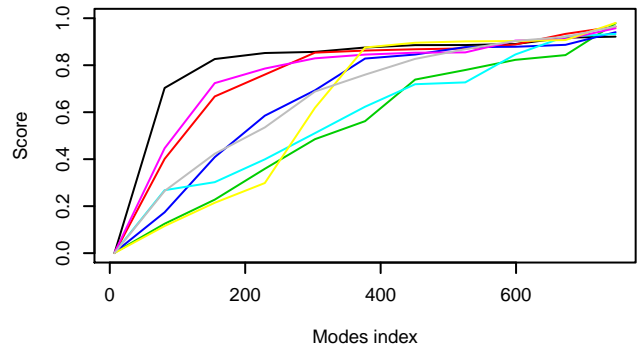
Cumulative overlap of CA modes of 1N55 (indiv_bend_upper)
