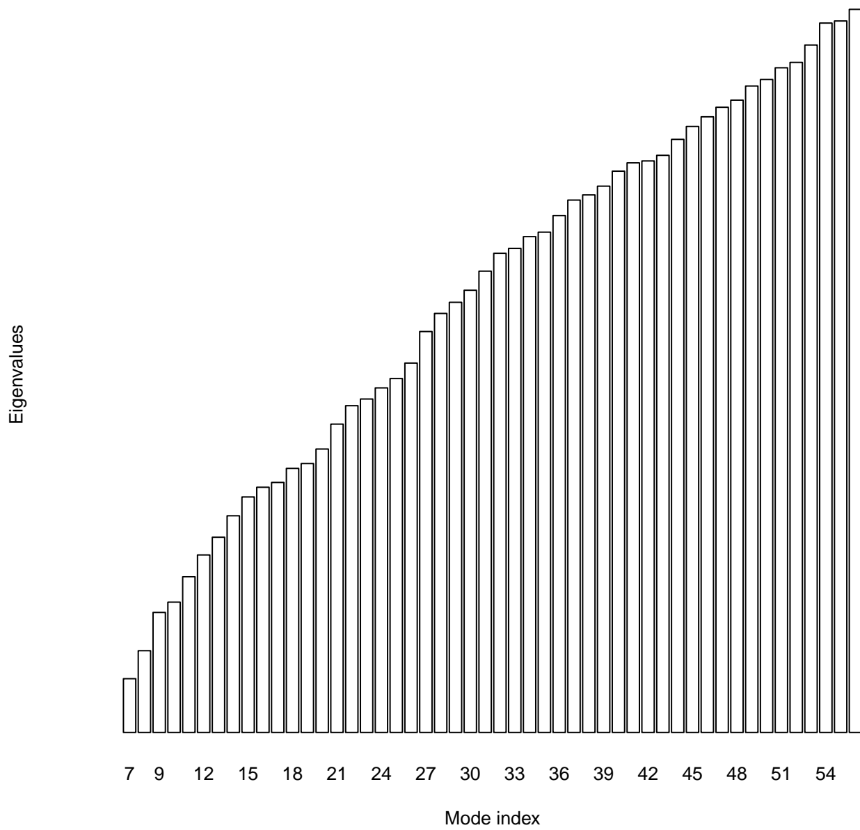
Eigenvalues plot for c.1.8.4_5.pdb
