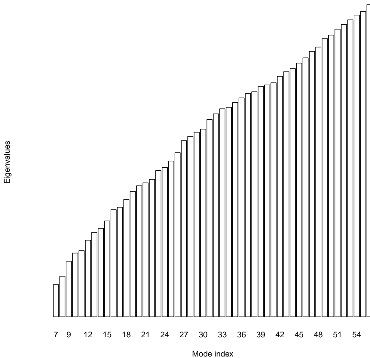
Eigenvalues plot for c.1.8.4_4.pdb
