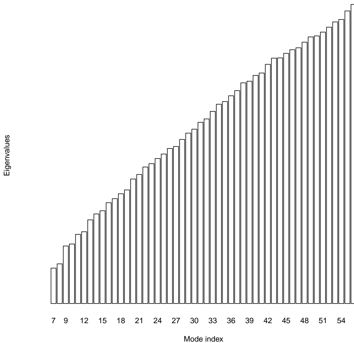
Eigenvalues plot for c.1.8.4_3.pdb
