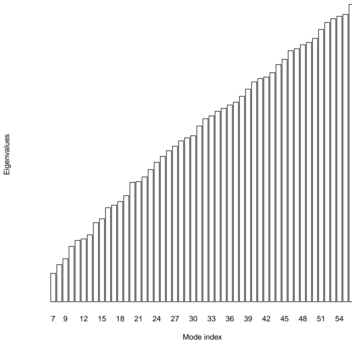
Eigenvalues plot for c.1.8.4_1.pdb
