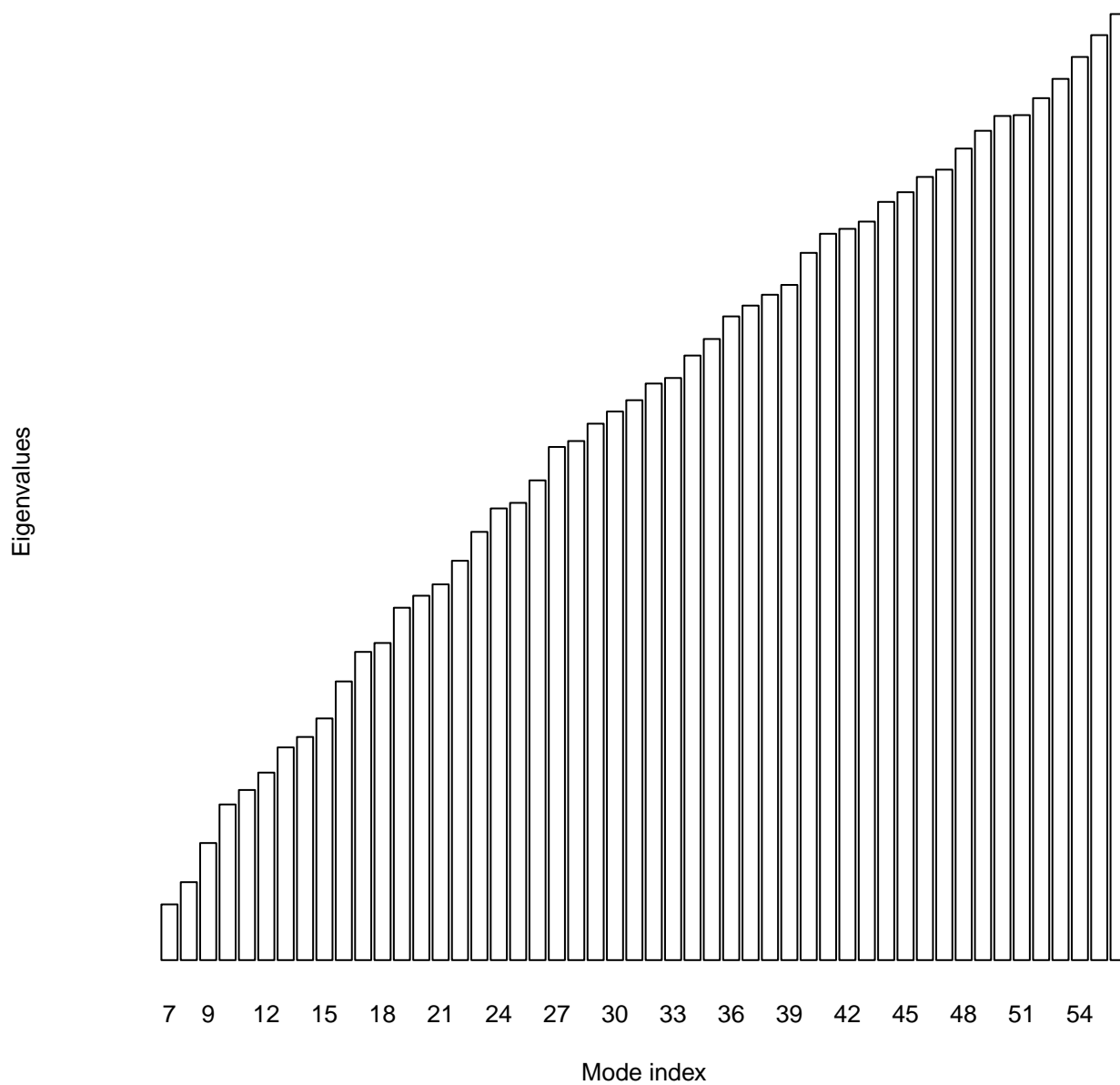
Eigenvalues plot for c.1.8.3_5.pdb
