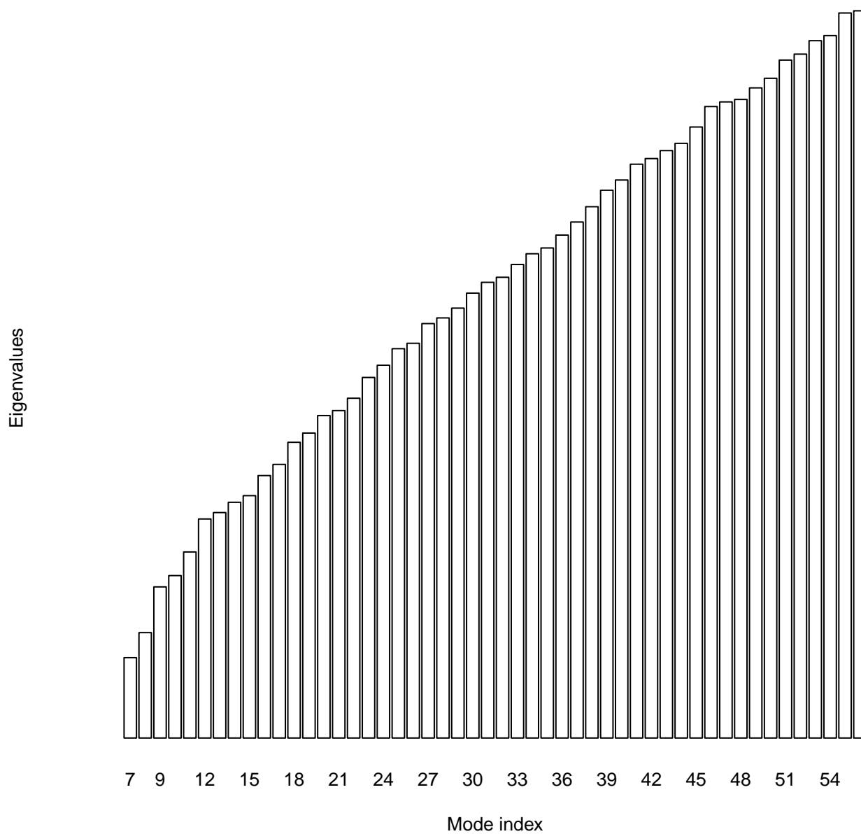
Eigenvalues plot for c.1.8.3_4.pdb
