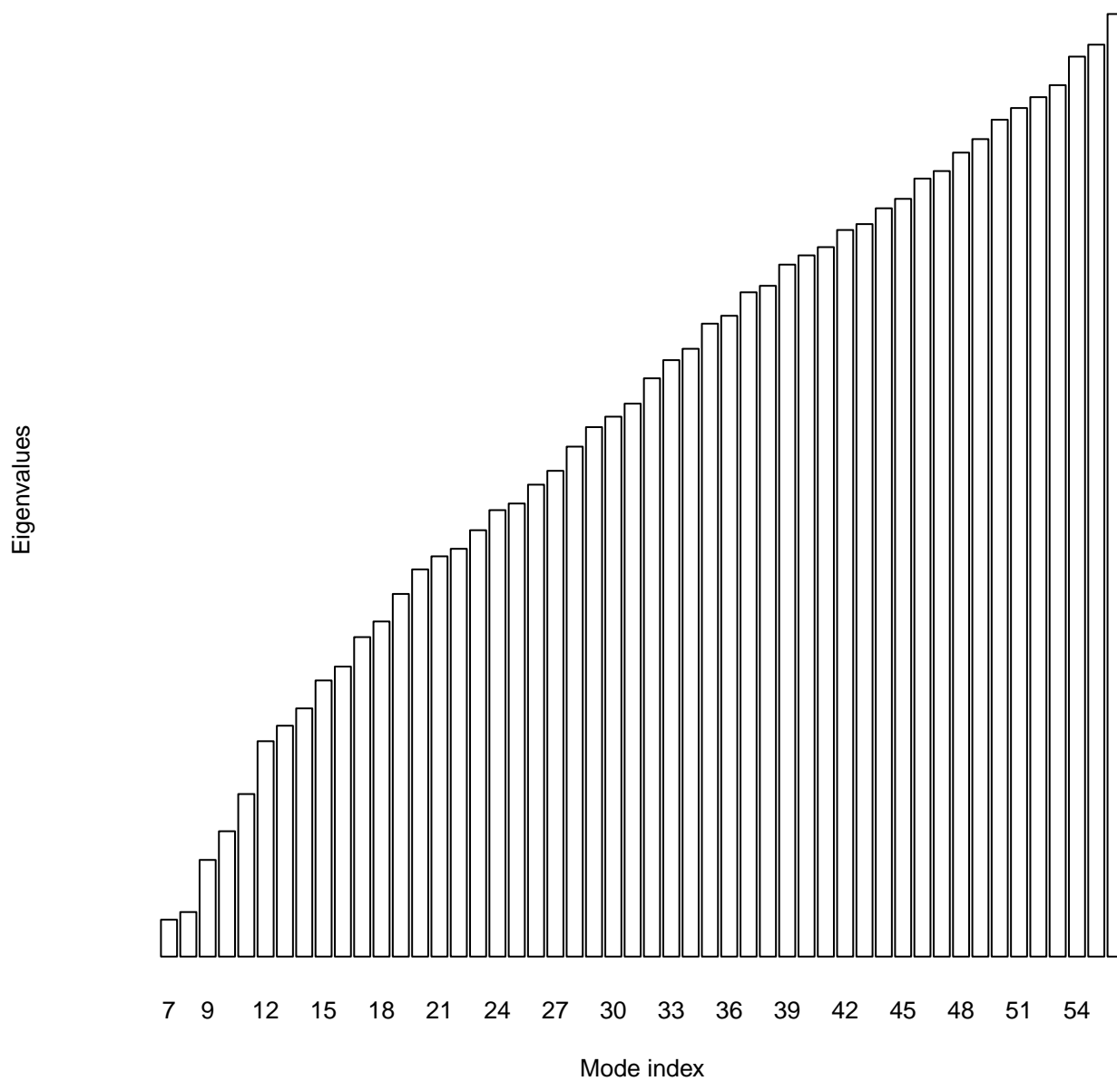
Eigenvalues plot for c.1.8.3_3.pdb
