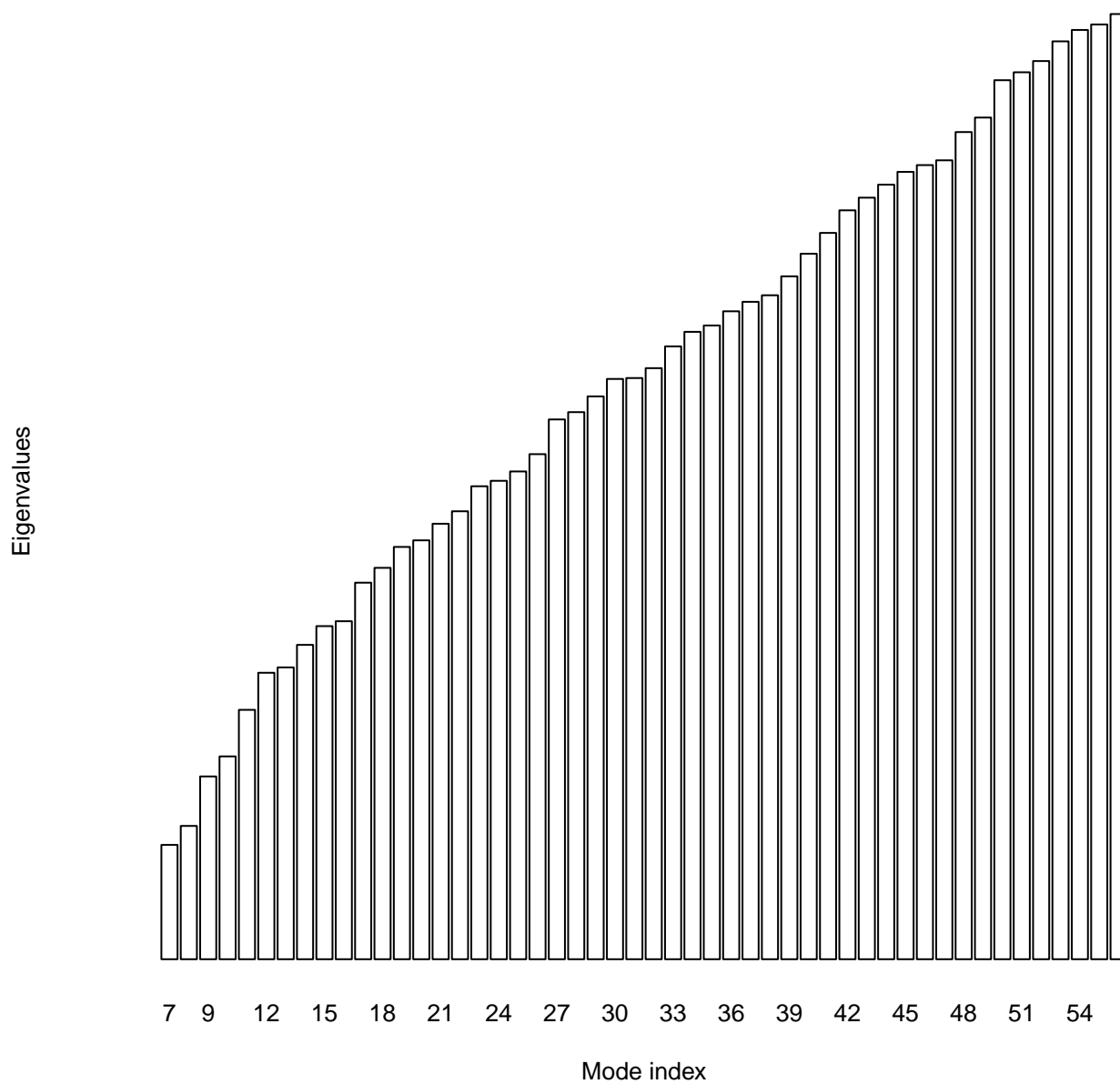
Eigenvalues plot for c.1.8.3_1.pdb
