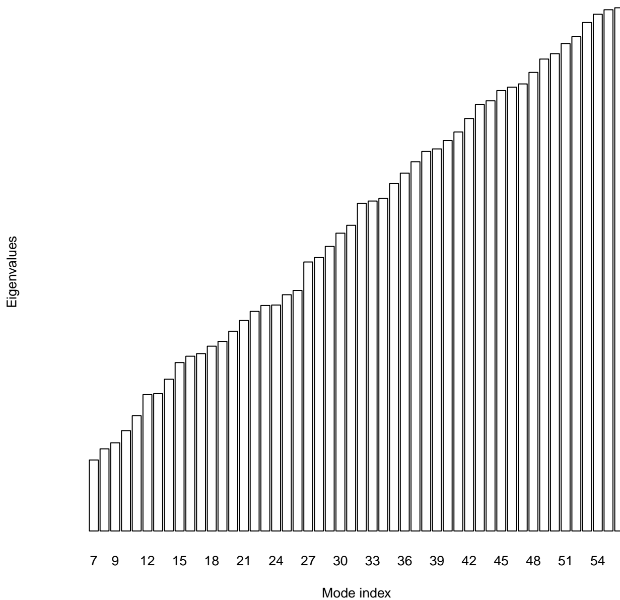
Eigenvalues plot for c.1.2.4_3.pdb
