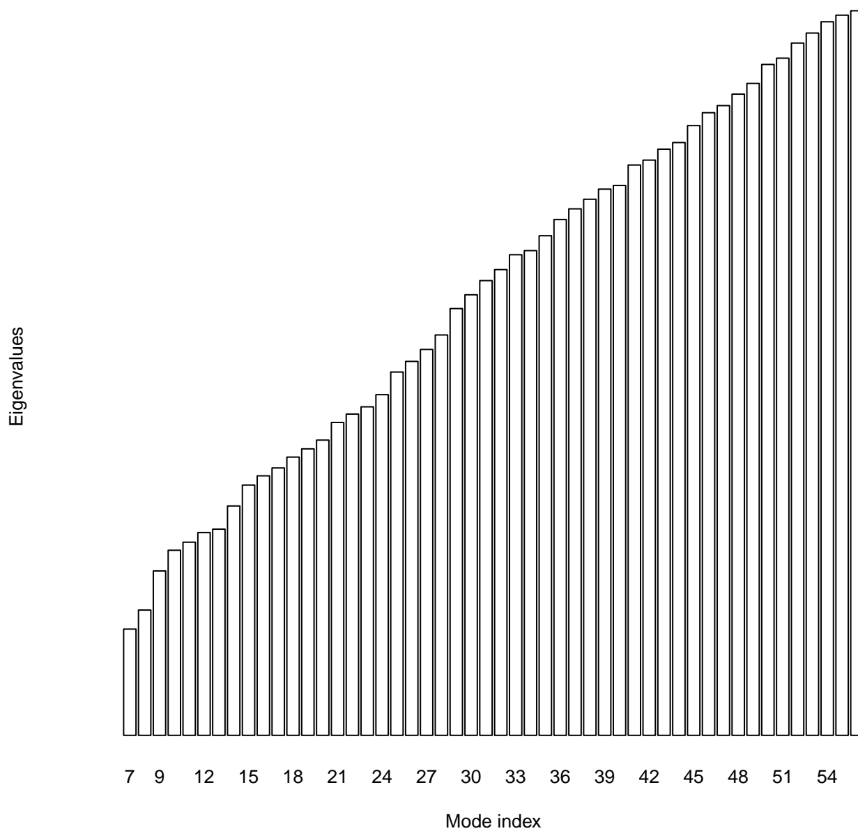
Eigenvalues plot for c.1.2.4_1.pdb
