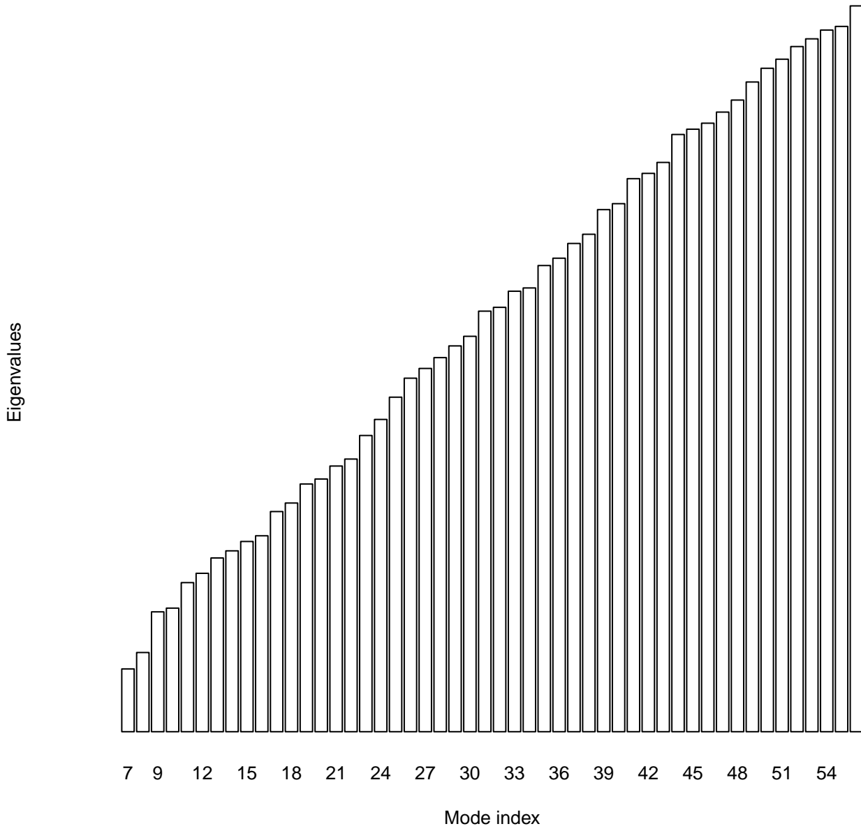
Eigenvalues plot for 1ake.pdb
