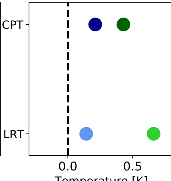
Temperature diff 2007-2018
