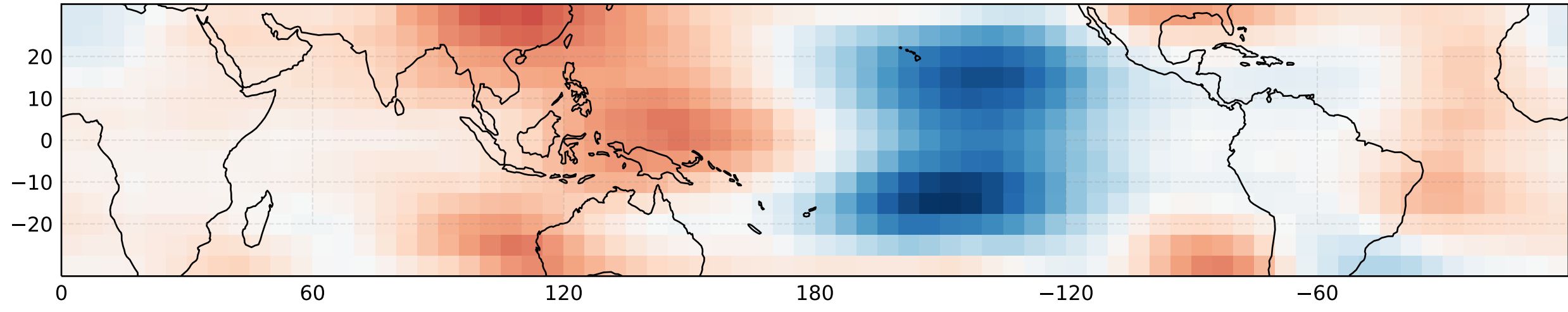
Difference El Niño - Mean, DJF 2007-2018 ERA5 Cold point temperature
